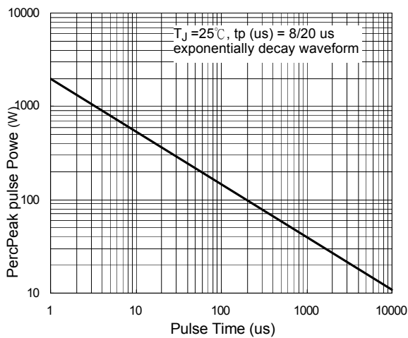
Figure 3. Power Dissipation versus Pulse Time
